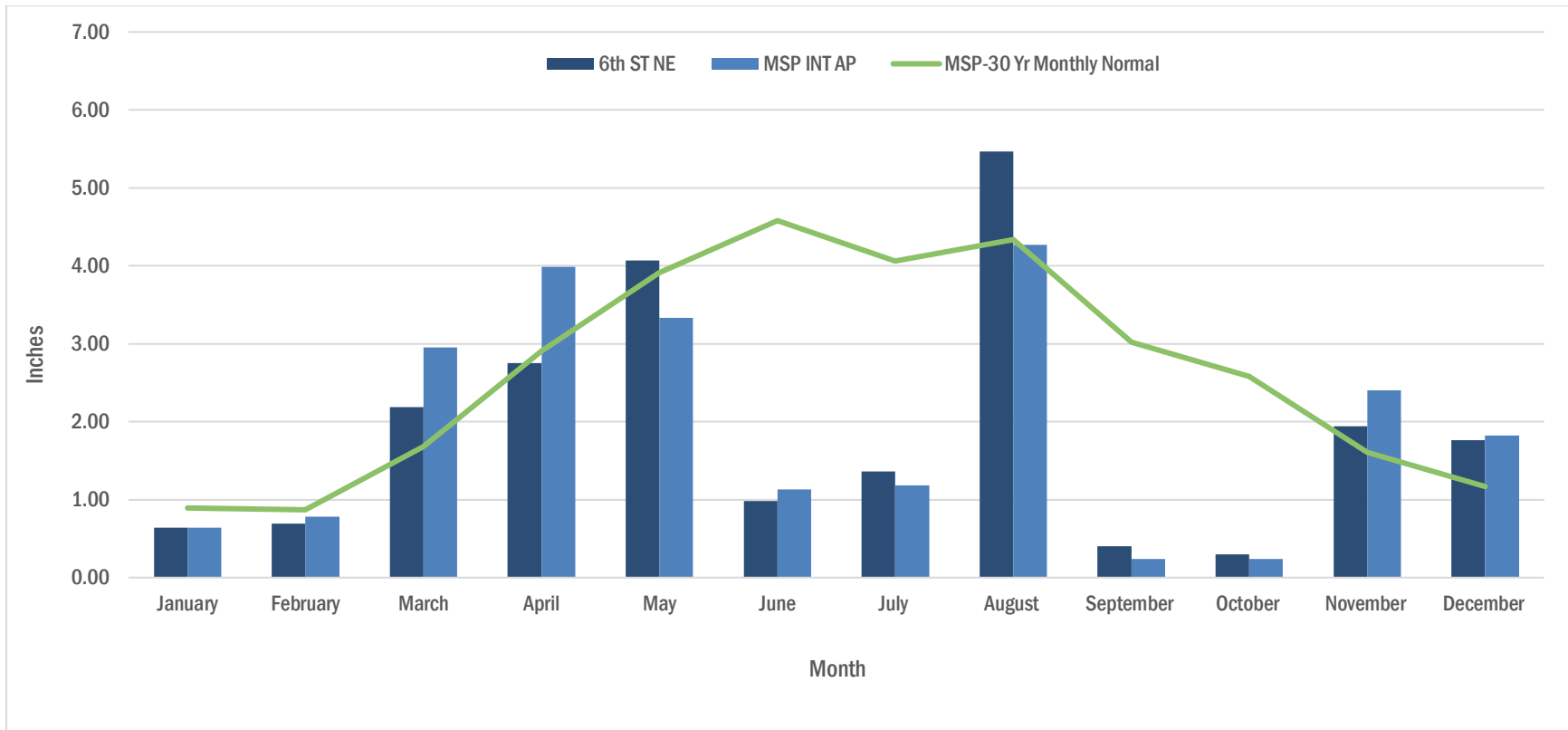
Figure 1. 2022 monthly precipitation totals at the 6 th ST NE rain gauge compared to 2022 monthly totals and 30-year monthly precipitation normals at the Minneapolis St. Paul International Airport.
