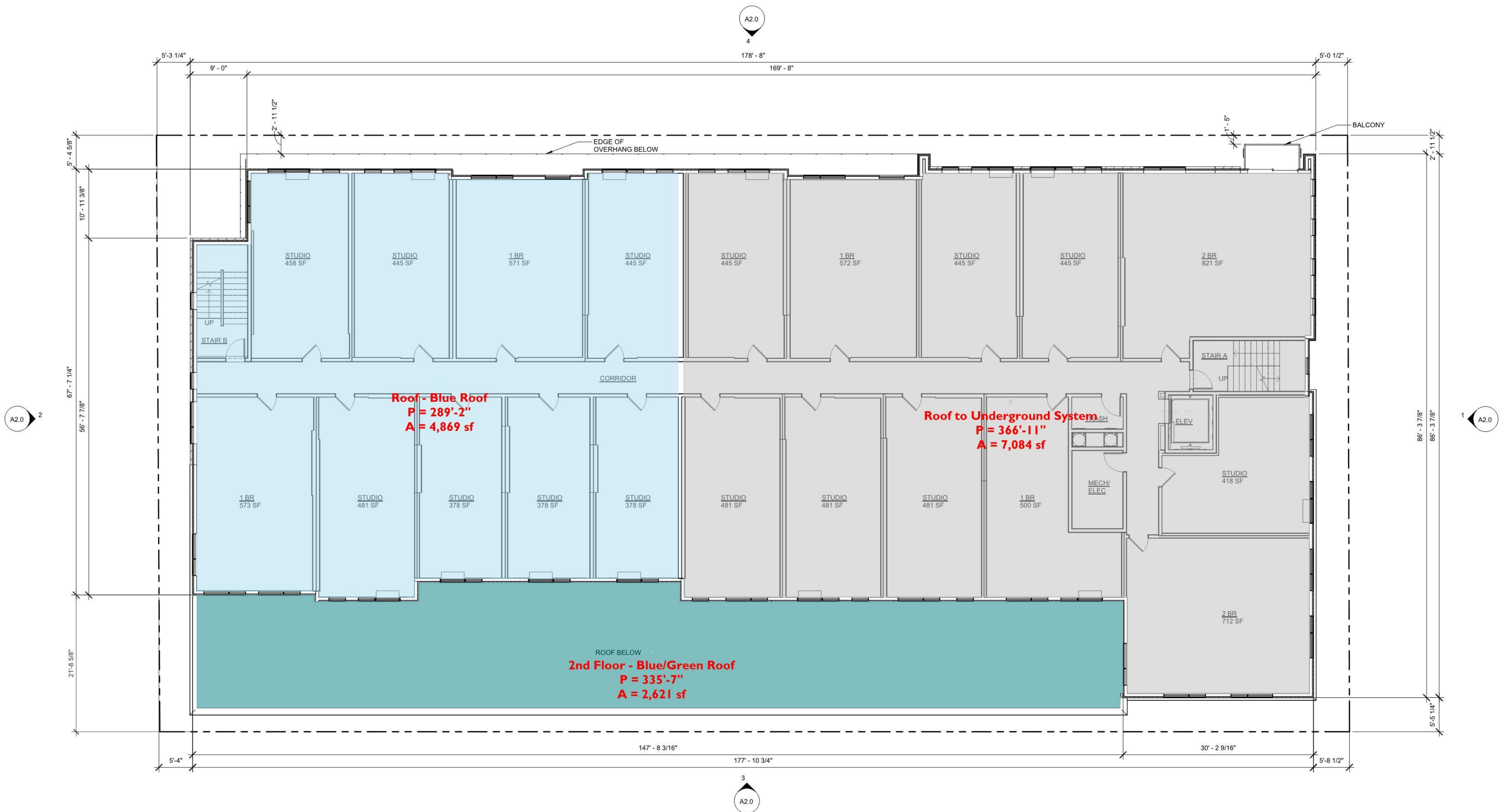
1 FLOOR PLAN - LEVEL 2 & 3 1/8" = 1'-0"
