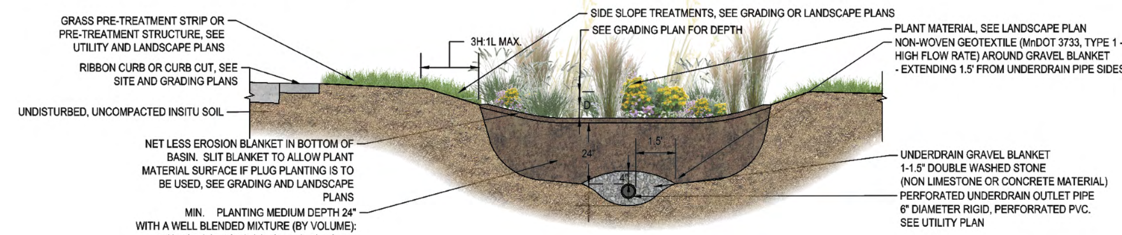
Rain Garden Section
